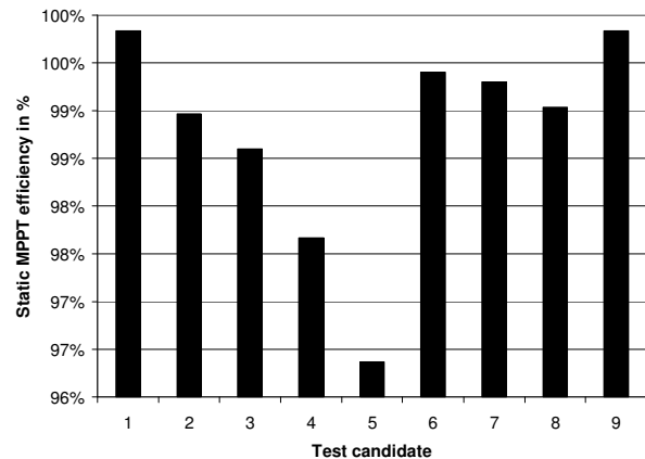
Graph 7: Overview on static MPPT efficiency
