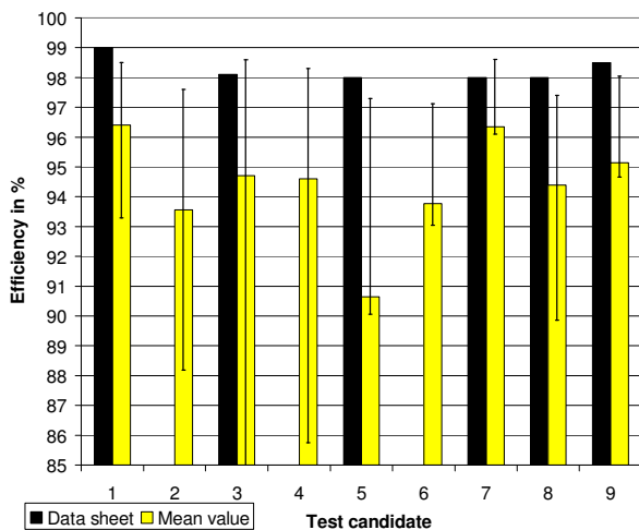
Graph 6 : DC-DC efficiency.
