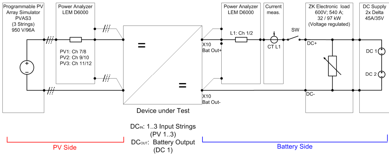
Graph 4 : Test setup for MPPT charge controllers at AIT 4
