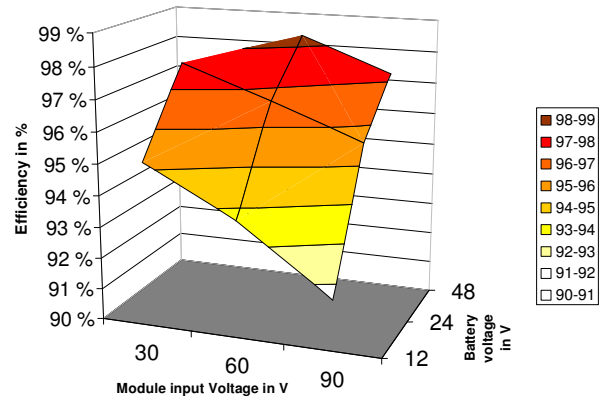
Graph 2: Weighted DC/DC conversion efficiency characteristics in dependency of the MPP and battery voltage.
