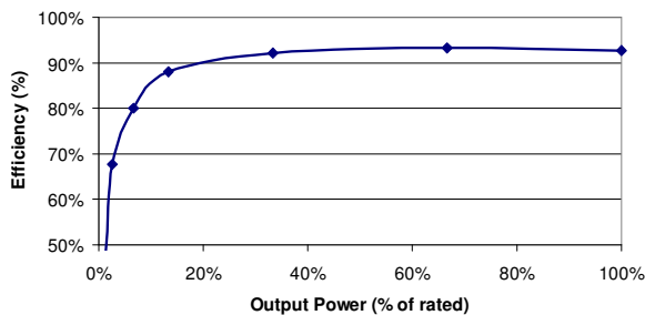
Graph 1: Typical dependency of the conversion efficiency on the output power
