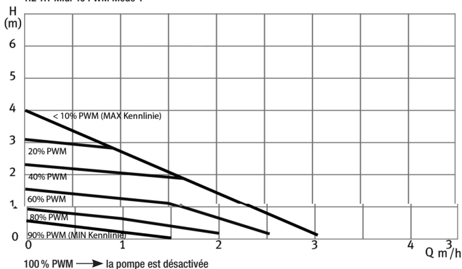
HE-HT Midi 40 PWM Mode 1
