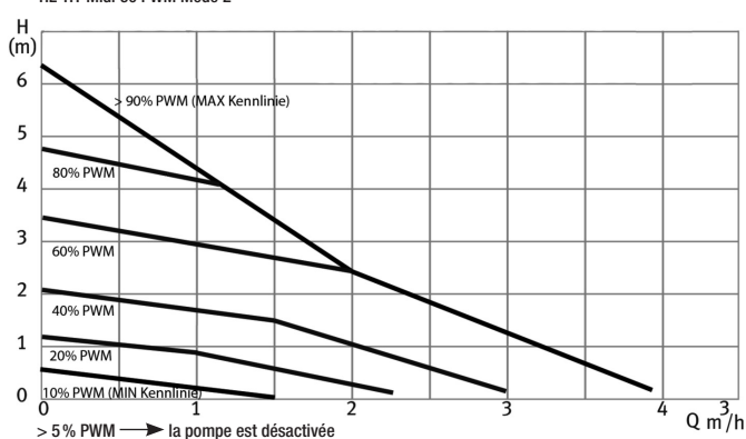
HE-HT Midi 60 PWM Mode 2
