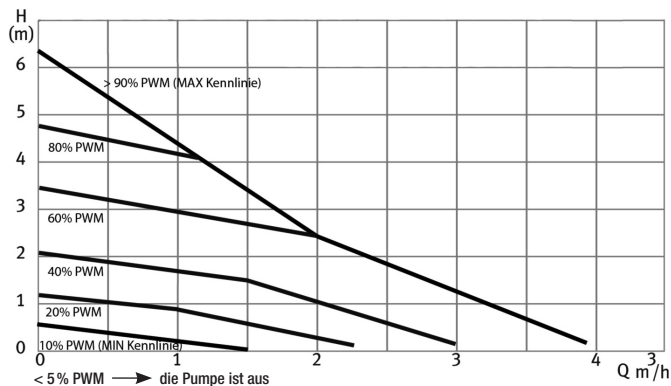
HE-HT Midi 60 PWM Mode 2
