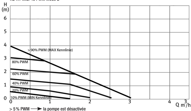
HE-HT Midi 40 PWM Mode 2
