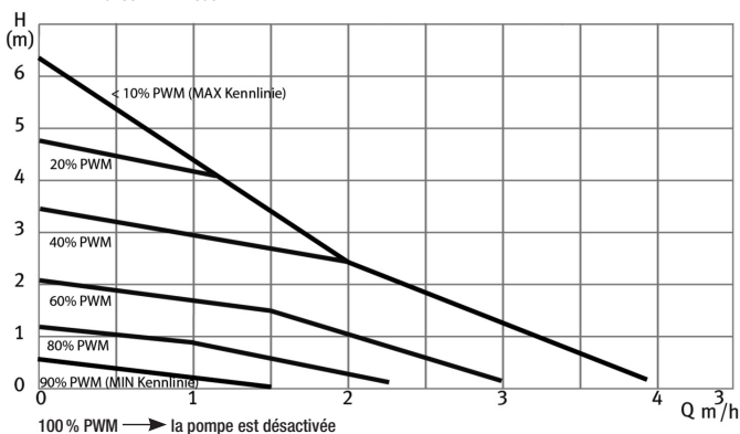
HE-HT Midi 60 PWM Mode 1
