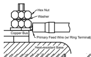
Recommended mounting
